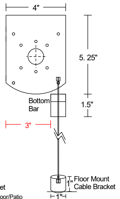
Under Eave w/ Floor Mount Cable Bracket
